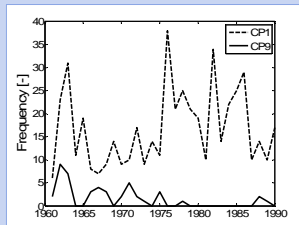
Fig. 3 (left): Decadal occurrence frequencies of the derived weather patterns using NCEP/NCAR reanalysis data for northern Burkina Faso (1961-1990); (right) Interannual variability of the wettest (driest) pattern CP1 (CP9).
