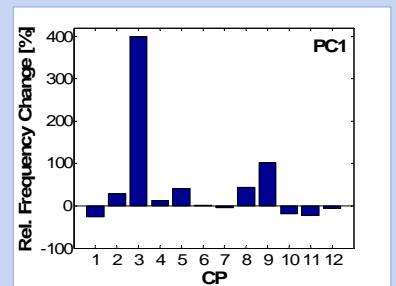
Fig. 4: Rel. change of the occurrence frequency of weather patterns of the future (2011-2040) compared to the past (1961-1990) in northern Burkina Faso.
