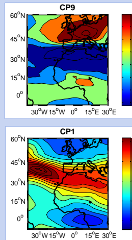
Fig. 2: Mean anomaly composites of the wettest (top) and driest CP (bottom) in the northernmost region of Burkina Faso using the eastward moisture flux in 500hPa.
